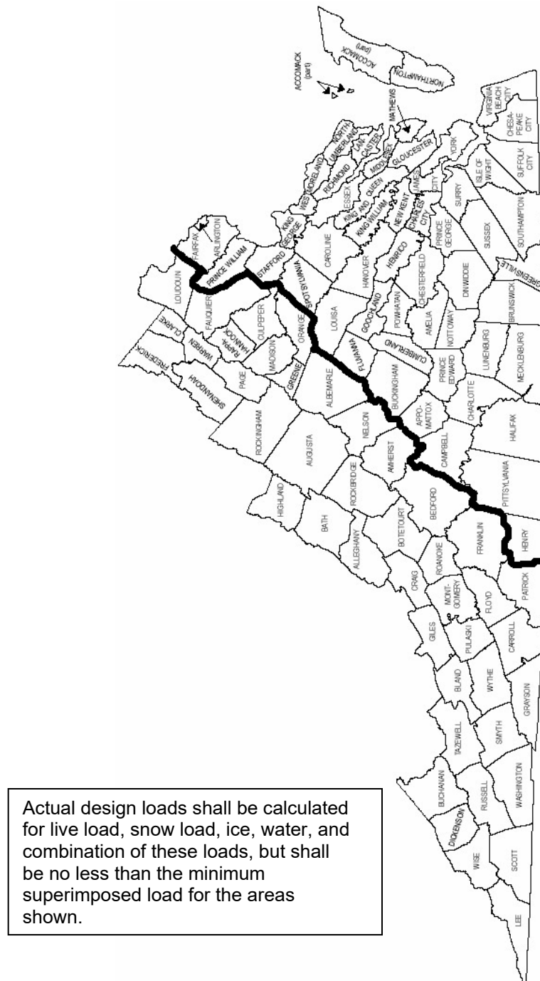
Figure 6.1.4.1 Minimum Superimposed Loads for Design of Low-Sloped Roofs
