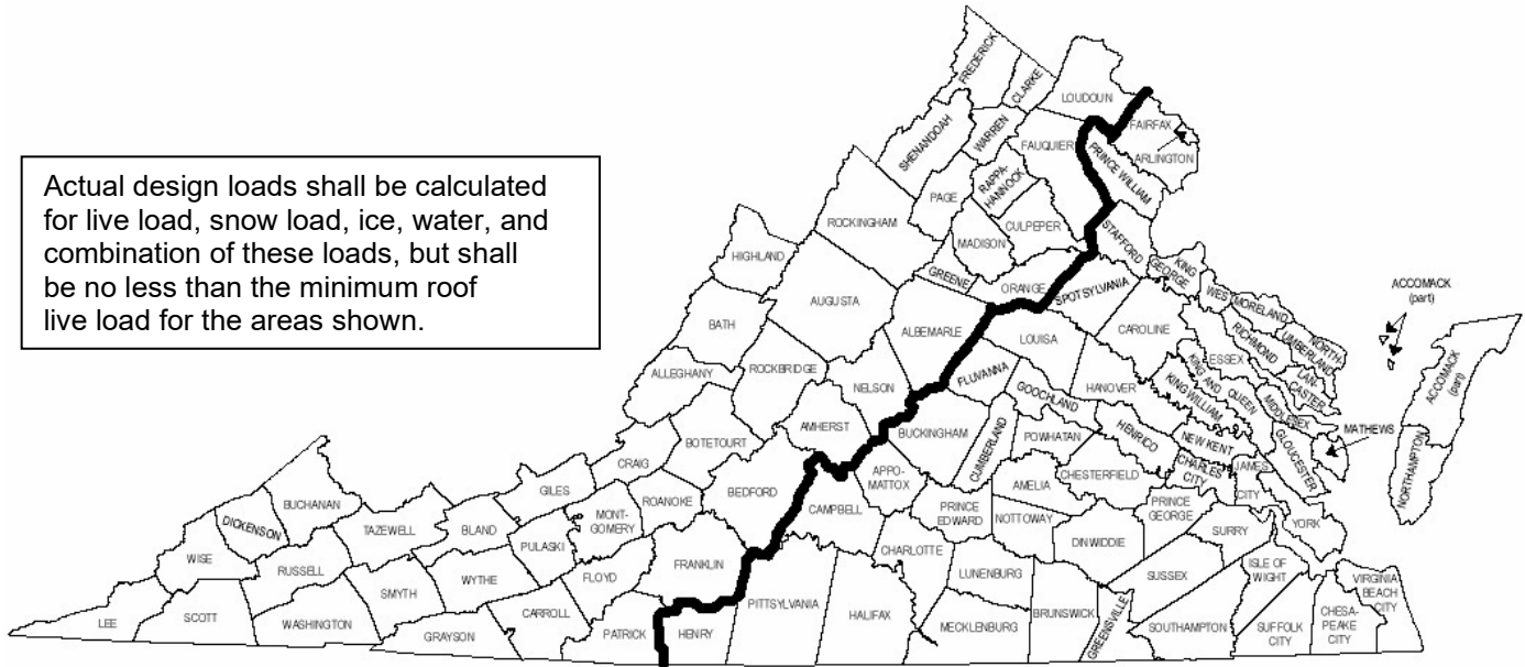
Figure 6.1.4.1 Minimum Roof Live Load for Design of Low-Sloped Roofs
